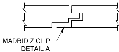
CONNECTION VIEW
